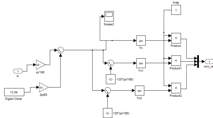
Fig.4.2.Phase Modulation of Control Angle
