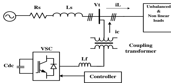
Fig.2.1 Basic DSTATCOM
