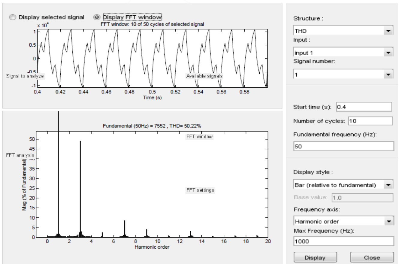
Fig.5.10 Waveform of distortion output current FFT without LCL passive filter and harmonic spectrum
