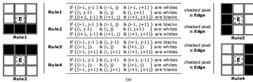
Figure 4 Fuzzy system rules
