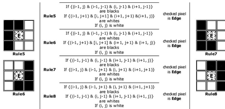
Figure 5 Fuzzy system rules
