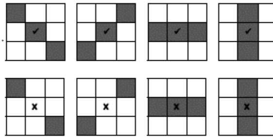
Figure 9 Strengthening and weakening of connected and separated edges
