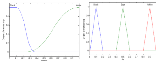
Figure 2 Input and output membership function
