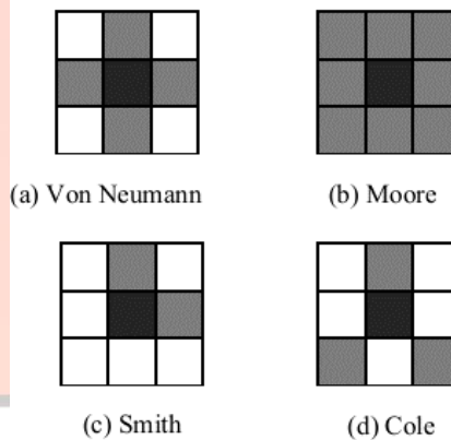
Figure 7 Types of neighborhood
