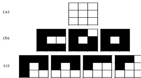
Figure 10 Penalty patterns. (a) Thick edge. (b) Noises. (c) Unwanted edges
