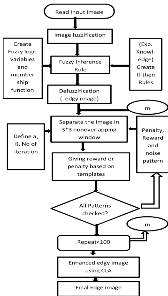
Figure 1 Proposed algorithm
