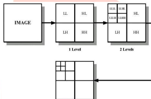
Fig. 3 2-D DWT for Image
