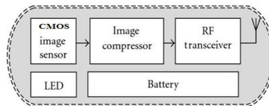
Fig. 1 Block diagram of Pill Cam
