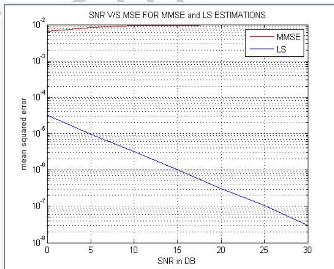
Figure 4 SNR vs MSE for 8-QAM
