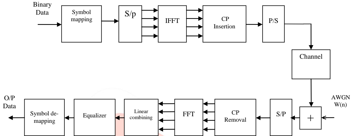
Figure 1 OFDM System Model
