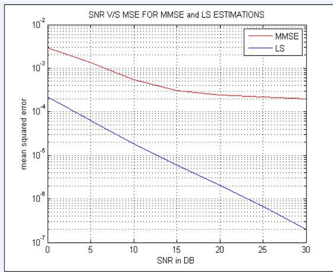
Figure 2 SNR VS MSE for BPSK
