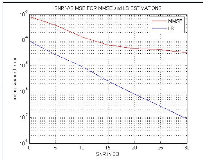
Figure 3 SNR vs MSE for QAM
