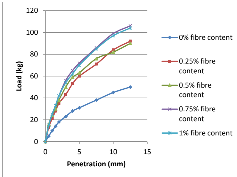
Fig 5. CBR curve for soil sample with different fiber content and fiber length=60mm
