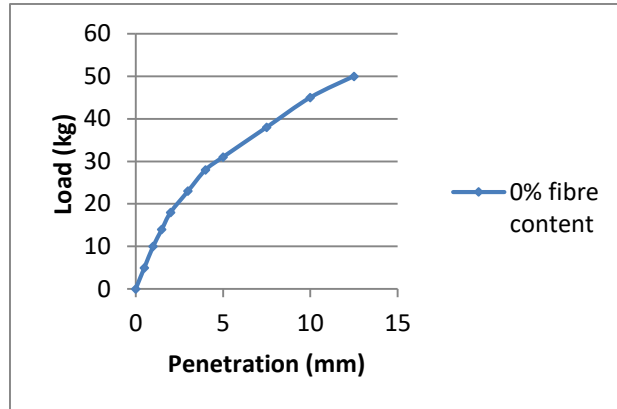
Fig 3: CBR Curve of Unreinforced Soil
