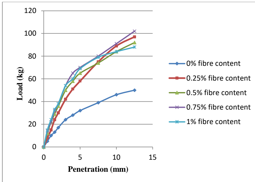
Fig 4. CBR curve for soil sample with different fiber content and fiber length=30mm
