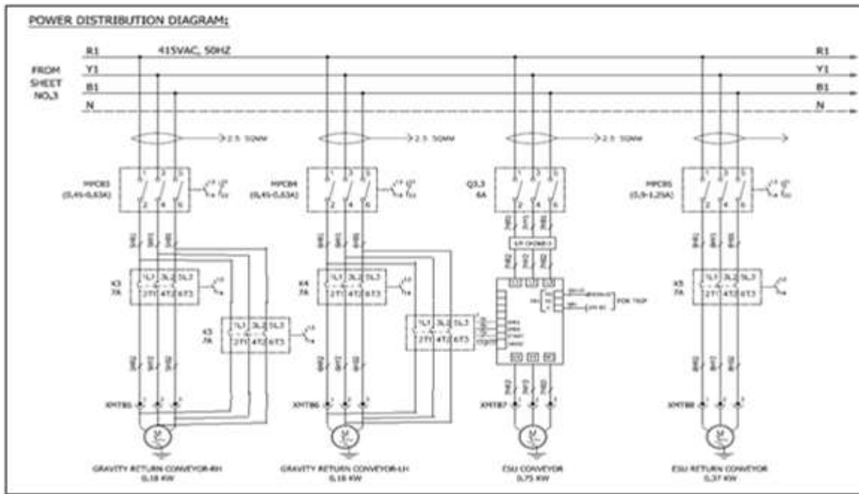
Fig :: power distribution diagram of modified gravity coater conveyor
