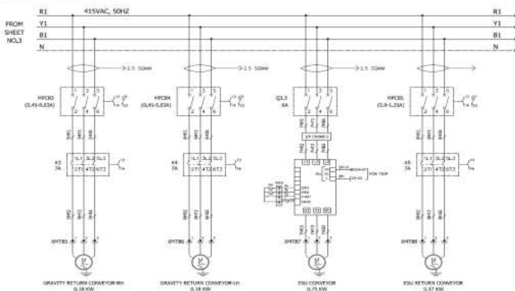
Fig : power distribution diagram of pre modified gravity conveyor
