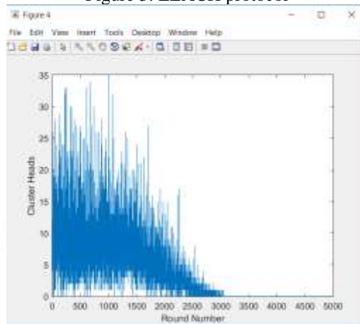
Figure 4: LEACH protocol
