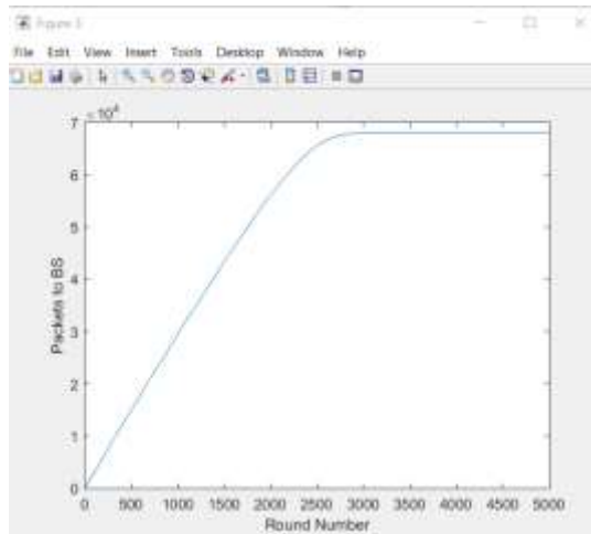
Figure 3: LEACH protocol
