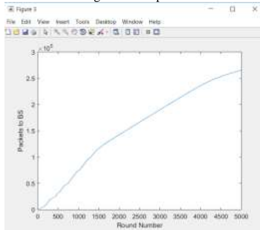
Figure 7: Proposed
