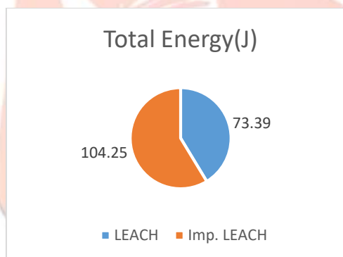
Figure 11: Energy Comparison
