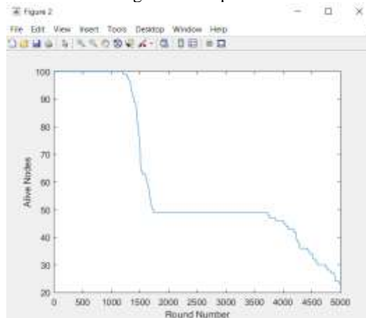
Figure 5: Proposed
