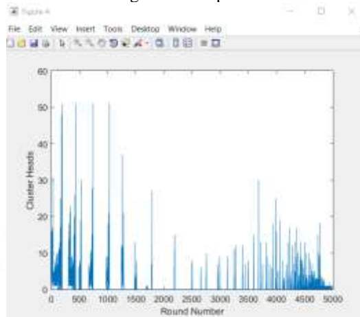
Figure 8: Proposed
