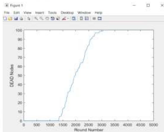
Figure 1: LEACH protocol
