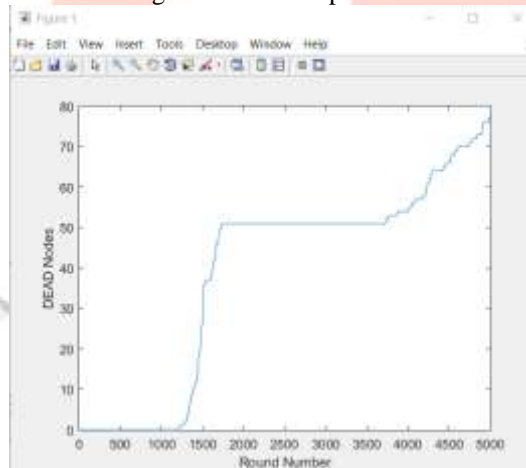
Figure 5: Proposed
