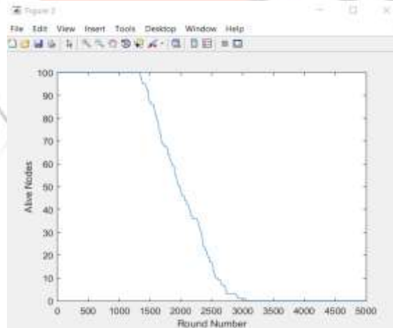
Figure 2: LEACH protocol
