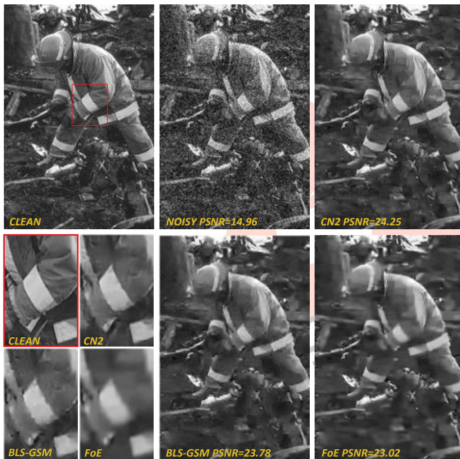
Figure 3: Denoising results on an image from the test set. The noisy image was generated by adding Gaussian noise with \sigma=50 to the clean image. Non-blind denoising results for the BLS-GSM, FoE, and convolutional network methods are shown. The lower left panel shows results for the outlined region in the upper left panel. The zoomed in region shows that in some areas CN2 output has less severe artifacts than the wavelet-based results and is sharper than the FoE results. CN1 results (PSNR=24.12) are visually similar to those of CN2.
