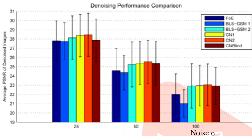
Figure 2: Denoising results as measured by peak signal to noise ratio (PSNR) for 3 different noise levels. In each case, results are the average denoised PSNR of the hundred images in the test set. CN1 and CNBlind are learned using the same forty image training set as the Field of Experts model (FoE). CN2 is learned using a training set with an additional sixty images. BLS-GSM1 and BLS-GSM2 are two different parameter settings of the algorithm in [1]. All methods except CNBlind assume a known noise distribution.
