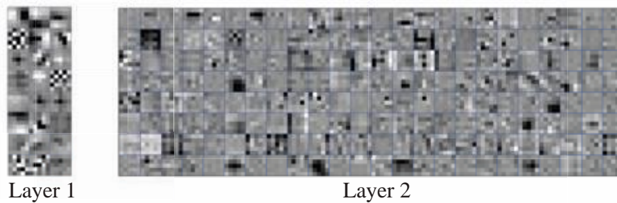
Figure 4: Filters learned for the first 2 hidden layers of network CNblind. The second hidden layer has 192 filters (24 feature maps 8 filters per map). The first layer has recognizable structure in the filters, including both derivative filters as well as high frequency filters similar to those learned by the FoE model [4, 6].
