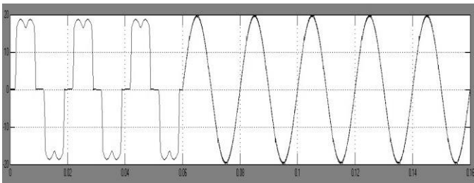
Fig. 6 Source current
