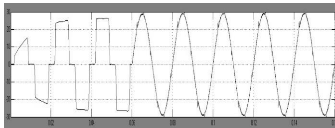
Fig. 11 Source current
