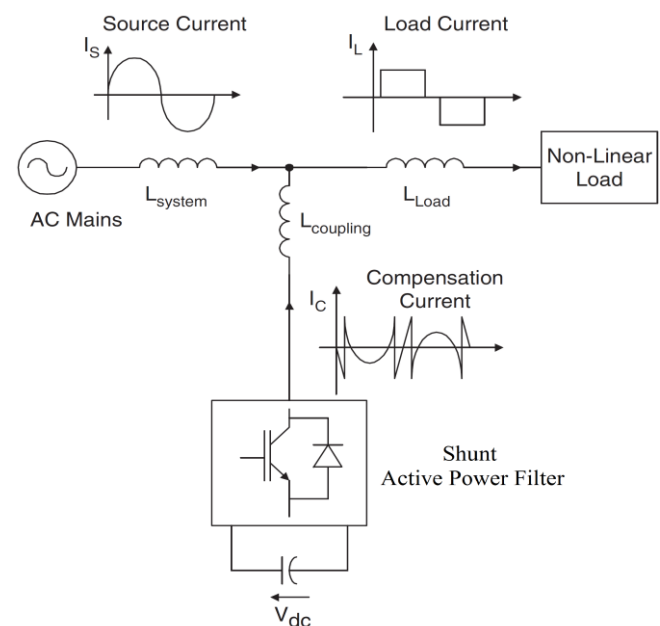
Fig. 1 Basic scheme of shunt active power filter
