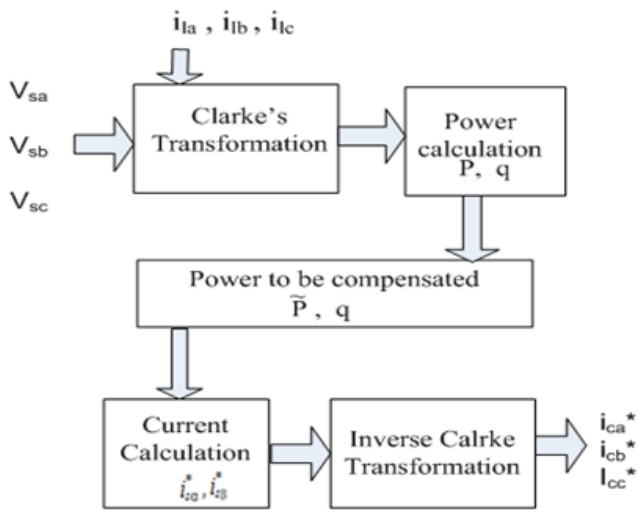
Fig. 5 Basic block diagram of p - q theory
