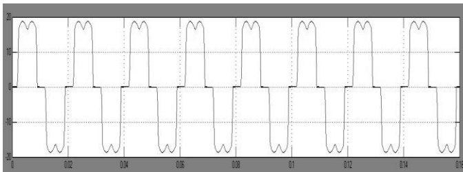
Fig. 8 Load current
