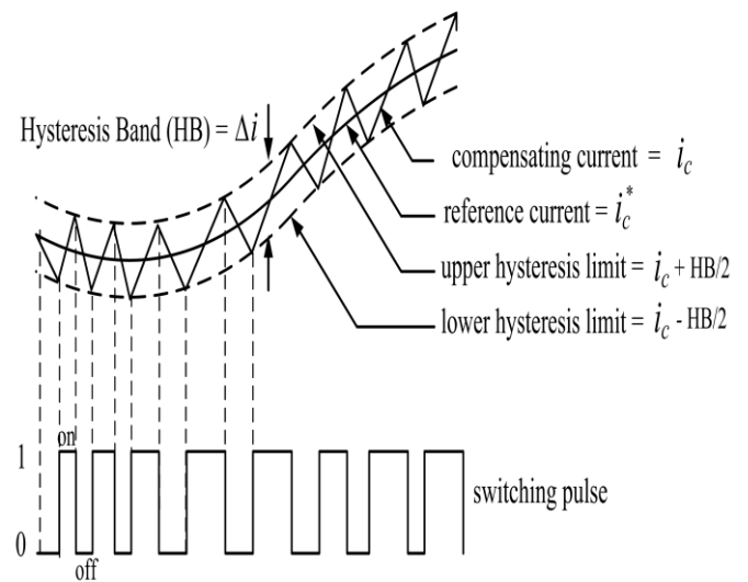
Fig. 3 Principle of hysteresis current control technique
