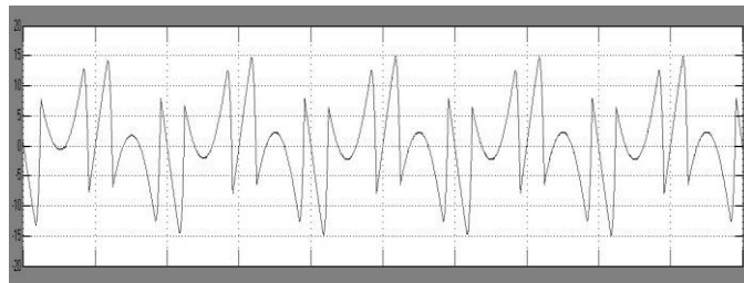
Fig. 12 Compensating current
