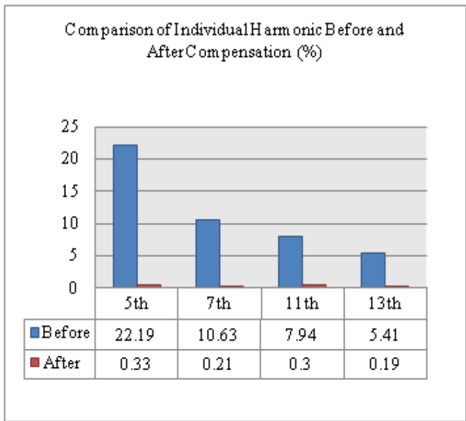
Fig. 10 Comparison of individual harmonics for Rectifier R load
