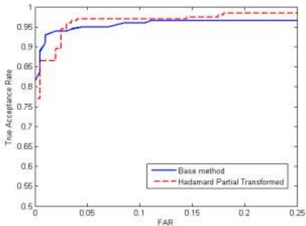
Fig.5: TAR vs. FAR Graph.
