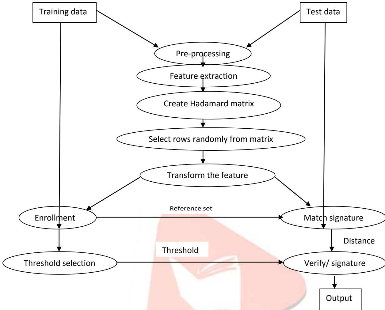
Fig 2: Flow Chart of the proposed Method
