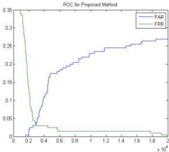
Fig. 6: ROC Curve for proposed method with low EER
