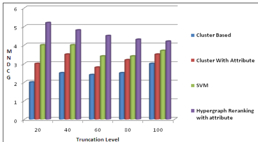
Chart -1: Performance Evaluation of our method with conventional methods.
