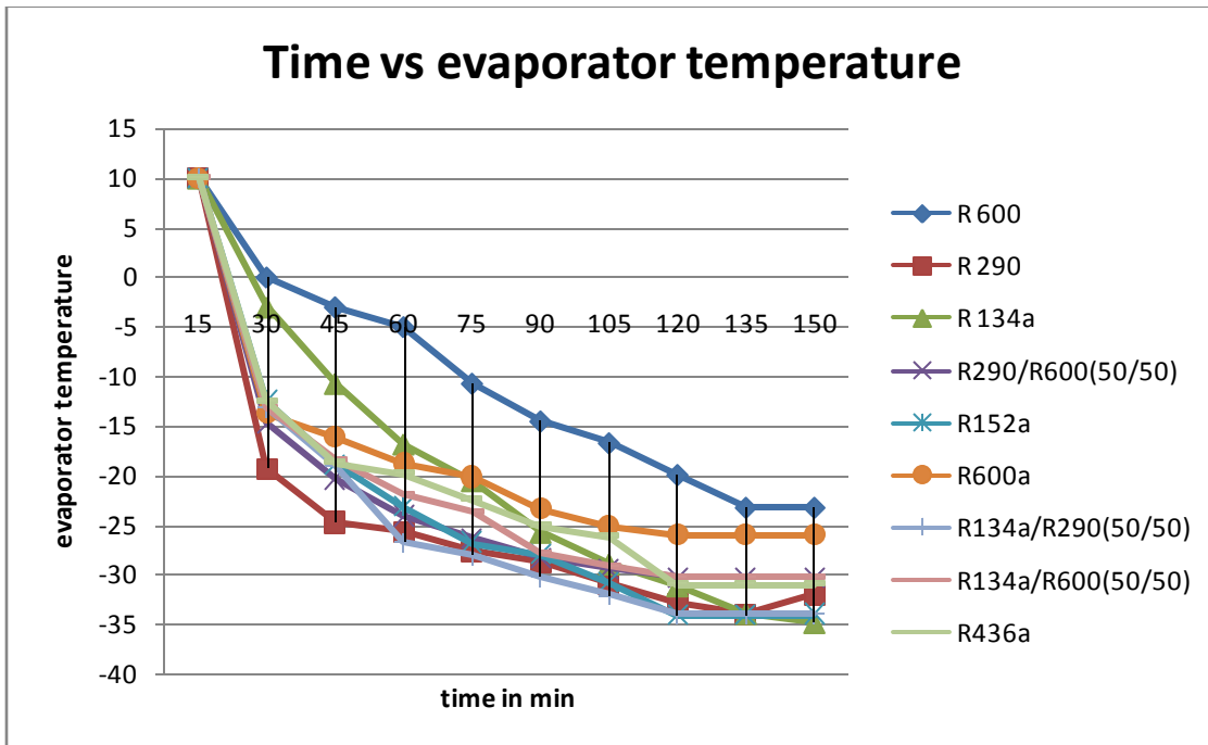
Fig 6.1 Time VS evaporator temperature
