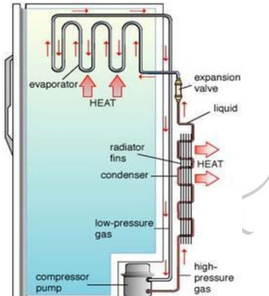
Fig. 1.4 Domestic Refrigerator
