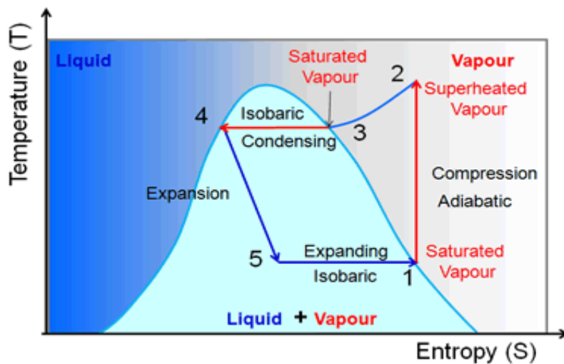
Fig. 1.2 T-S diagram of VCRS system
