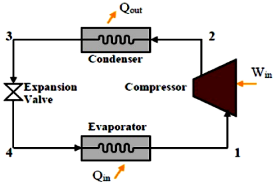
Fig. 1.1 VCRS system
