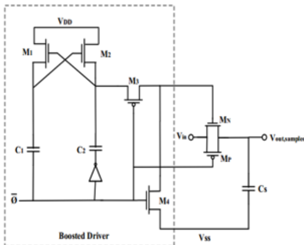
Fig5. S/H circuit with boosted driver
