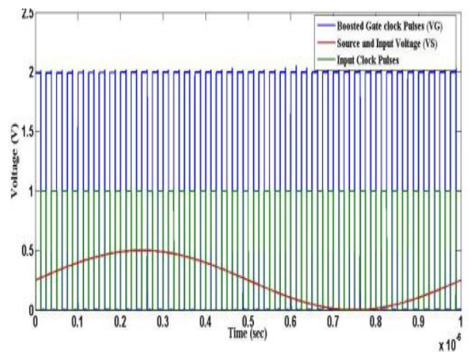
Fig6. Input clock pulses, boosted driver output and the input voltage
