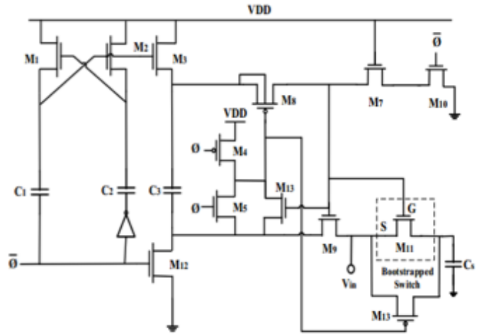
Fig2. S/H with bootstrapped circuit
