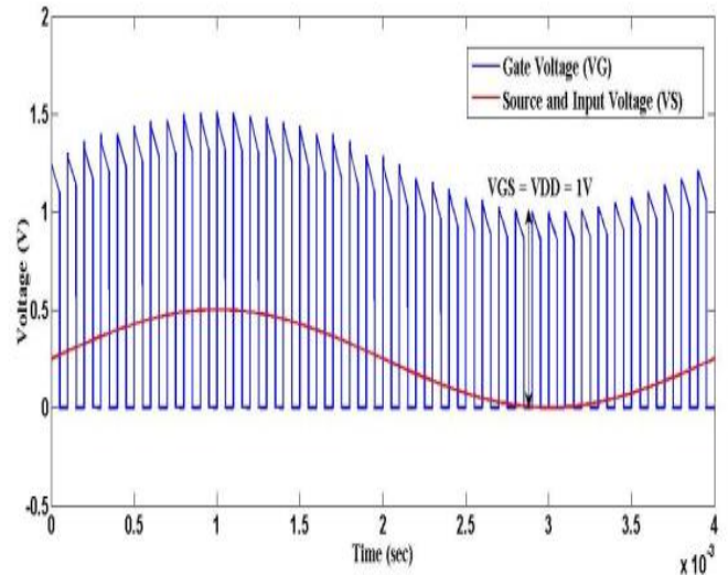
Fig4: M11 Input signal with the clock pulses formed on G for the low-power bootstrapped S/H circuit without multiplier circuit.
