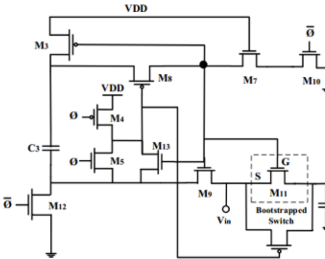
Fig3: Low-power bootstrapped S/H circuit without multiplier circuit.
